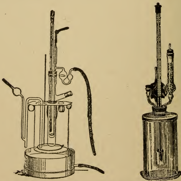
Figs. 86 and 87. APPARATURES FOR DETERMINING MOLECULAR WEIGHT
